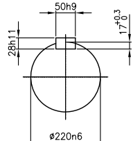
OUTPUT SHAFT
