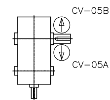
CR CV-05A/B SHAFT ARRANGEMENT & DIRECTION of ROTATION
