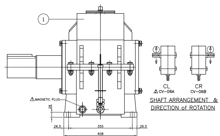
INPUT SHAFT OUTPUT SHAFT
