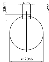
OUTPUT SHAFT
